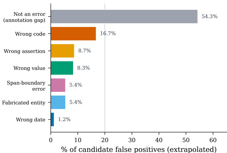
C Hallucination taxonomy on candidate FPs
